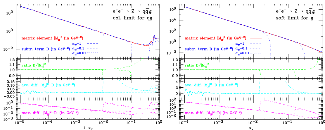
Figure 1: Matrix element squared |M_R|^2 (upper plots, solid line) and the subtraction terms D (upper plots, dashed/dotted/dot-dashed lines) for the process e^+(p_1)e^-(p_2) \rightarrow Z \rightarrow q(p_3)\bar{q}(p_4)g(p_5) as a function of 1 - x_{\bar{q}} = (p_3.p_5)/(p_1.p_2) and x_g = 1 - (p_3.p_4)/(p_1.p_2) in figures (a) and (b), respectively. Also plotted are the ratio D/|M_R|^2 , the difference |M_R|^2 - D (averaged over 100 random points per bin) and the maximal difference \max(|M_R|^2 - D) per bin. The dashed lines include the dipoles for each point in phase space, \alpha_{ff} = 1 , while for the dotted \alpha_{ff} = 0.1 and dot-dashed \alpha_{ff} = 0.01 the phase space for the dipoles has been restricted to the collinear/soft regions.
