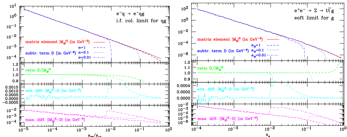
Figure 2: Matrix element squared |M_R|^2 (upper plots, solid line) and the subtraction term D (upper plots, dashed/dotted/dot-dashed lines) for (a) the process e^-(p_1)q(p_2) \rightarrow e^-(p_3)q(p_4)g(p_5) as a function of s_{25}/s_{12} = (p_2 \cdot p_5)/(p_1 \cdot p_2) and (b) the process e^+(p_1)e^-(p_2) \rightarrow Z \rightarrow t(p_3)\bar{t}(p_4)g(p_5) as a function of x_g = 1 - (p_3 \cdot p_4)/(p_1 \cdot p_2) . Also plotted are the ratio D/|M_R|^2 , the difference |M_R|^2 - D (averaged over 100 random points per bin) and the maximal difference \max(|M_R|^2 - D) per bin. The dashed lines include the dipoles for each point in phase space, \alpha = 1 , while for the dotted \alpha = 0.1 and dot-dashed \alpha = 0.01 the phase space for the dipoles has been restricted to the collinear/soft regions.
